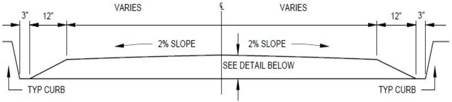
SPEED TABLE SECTION A-A NTS
