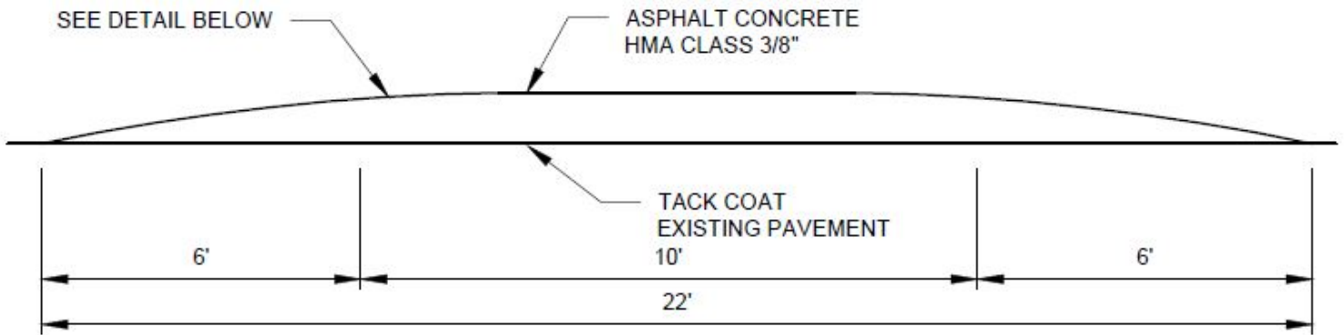
SPEED TABLE SECTION B-B NTS
