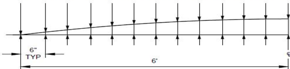
SPEED TABLE DETAIL (TYP) NTS
